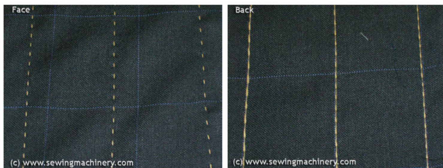
Stitch sample, note the difference in the stitch spacing on each of the 3 sewn lines
