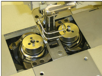
Walking foot & 2x Large Vertical Axis Hooks
