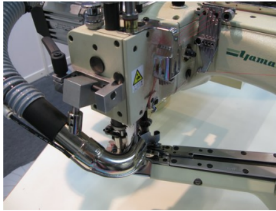
"Magic Dry" 4 Needle Flatseamer for Full Overlapping
