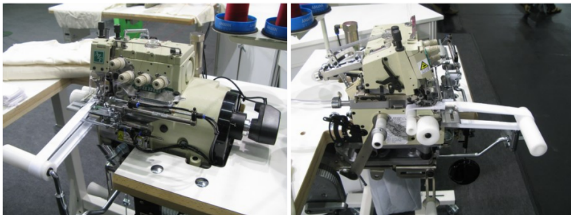
2 Needle- 4 Thread Small Cylinderarm Overlock machine with Variable Top Feeder and Elastic tension Roller System for attaching Collar
