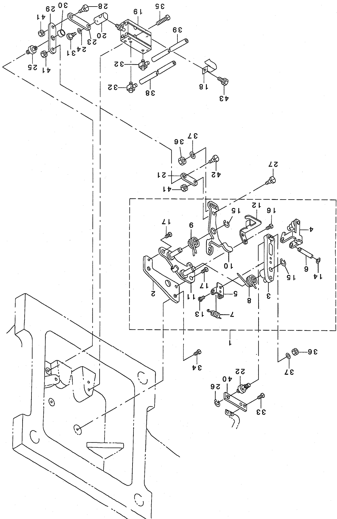
10. THREAD TRIMMER MECHANISM COMPONENTS (2) 糸切り関係 (2)
