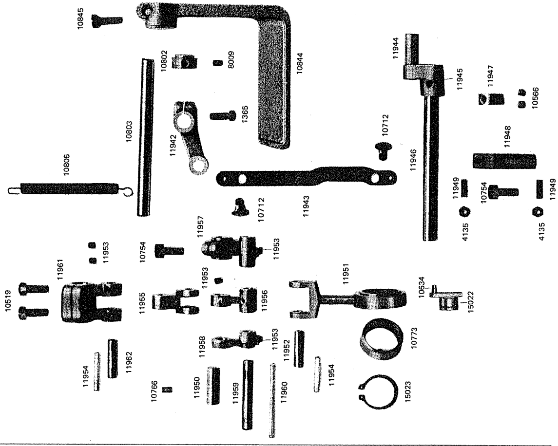
REVERSE FEEDING
