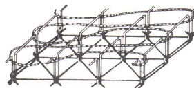
STITCH TYPE 607 FOUR NEEDLE SIX THREAD INTERLOCK
